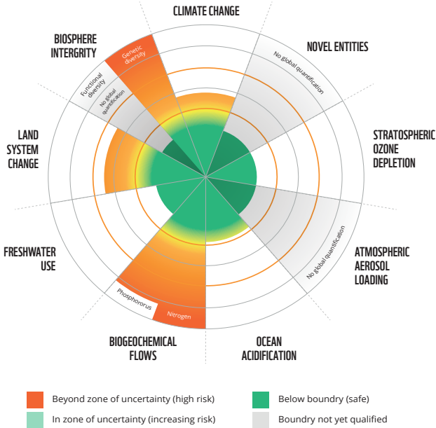
FIGURE 4A The planetary boundaries framework describing the upper limits of environmental impact from all human activities at the global scale. Source: Whitmee et al. 2015
